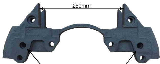
Counter Sunk Holes
